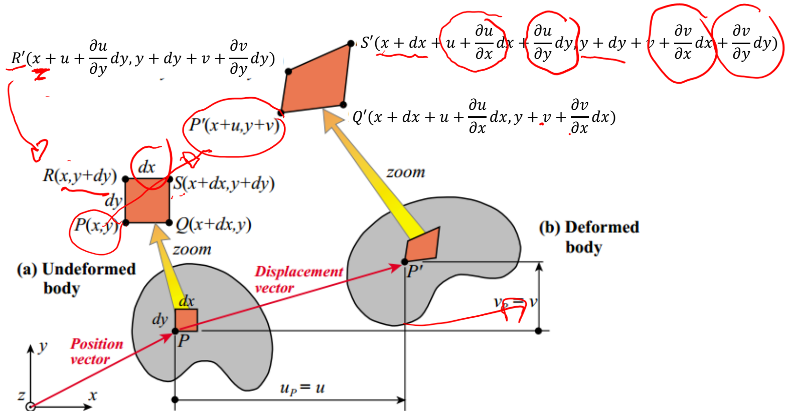
Connecting strains to displacements: 2D view used for visualization convenience.
